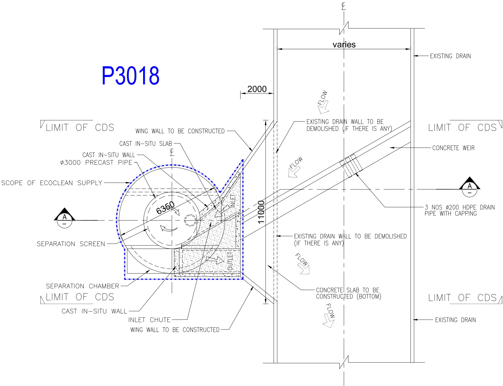
PLAN SECTION B-B
