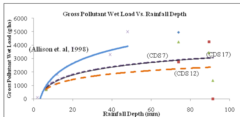
Figure 4. Comparison of Malaysia Condition and Australian Condition for Relationship of Gross Pollutant Wet Load against Rainfall Depth.
