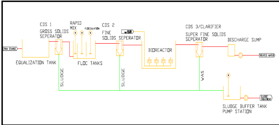
AFBR PROCESS DIAGRAM
